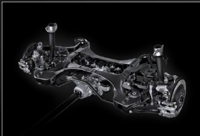
Rear suspension (2.4L petrol) with AVS.
